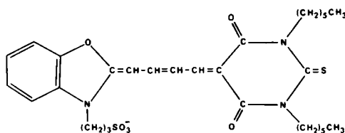
FIGURE 1 The structure of the merocyanine dye used in the experiments illustrated in Figs. 2 and 3.
